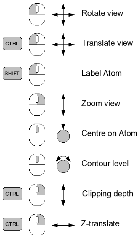
Figure 1: Mouse Controls in Coot
