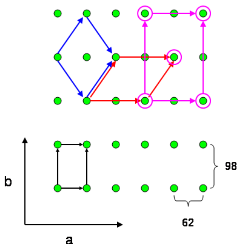
Figure 1. The action of matrix \mathbf{M} on the original lattice of the ( P212121 native) lego cell is shown. The original orthorhombic cell is shown in black. The monoclinic cell obtained after application of matrix \mathbf{M} is shown in red. A cell reduction of the red unit cell results in the blue SeMet1 cell. The C-centered cell of the SeMet2 derivative is shown in pink. The view is along the original c axis.
